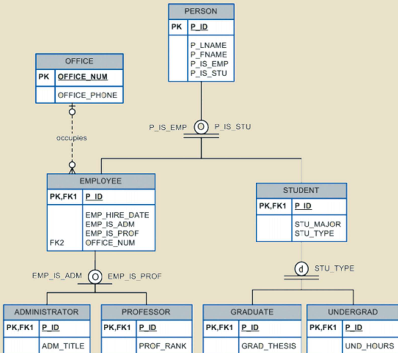
FIGURE 5.4 SPECIALIZATION HIERARCHY WITH OVERLAPPING SUBTYPES
